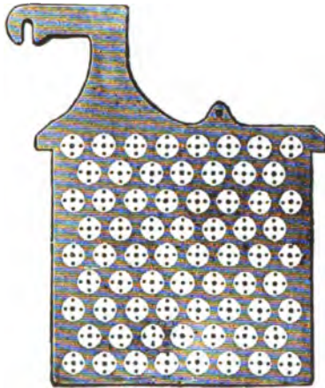
FIG. 450.—One Plate, or "Grid," of a Type of Storage Cell constructed by inserting buttons or ribbons of the proper chemical substances in perforations. Some such cells use crimped ribbons of metallic lead for inserting in the perforations, others pure red lead or other suitable material.
